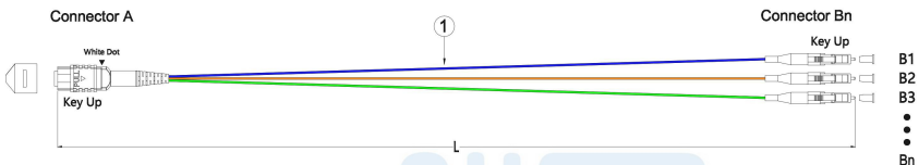
0.9mm Fanout with equal length
