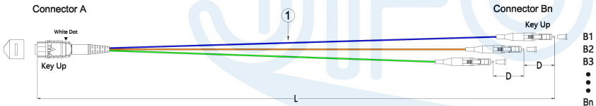
0.9mm Fanout with unequal length
