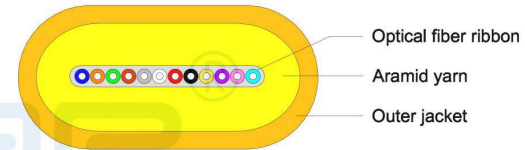
Ribbon Cable
