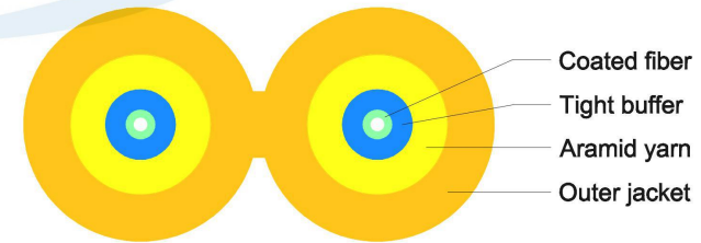
Cable Profile View
